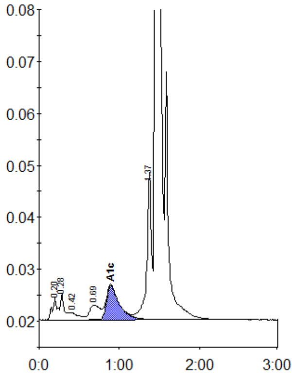
Peak table - ID: 10404372
